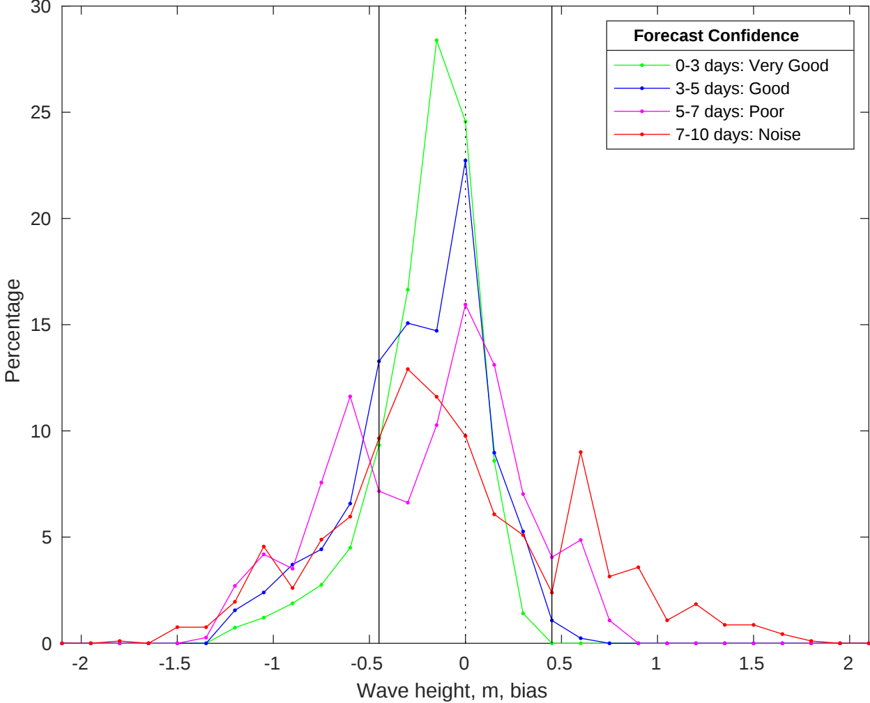
NDBC 42020 vs CMEMS Waves Bias Histogram: 19-May-2025
