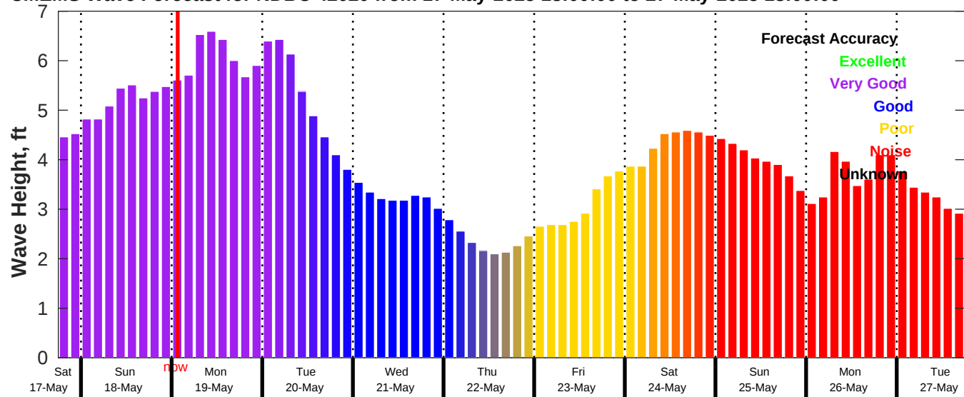
CMEMS Wave Forecast for NDBC 42020 from 17-May-2025 18:00:00 to 27-May-2025 18:00:00
