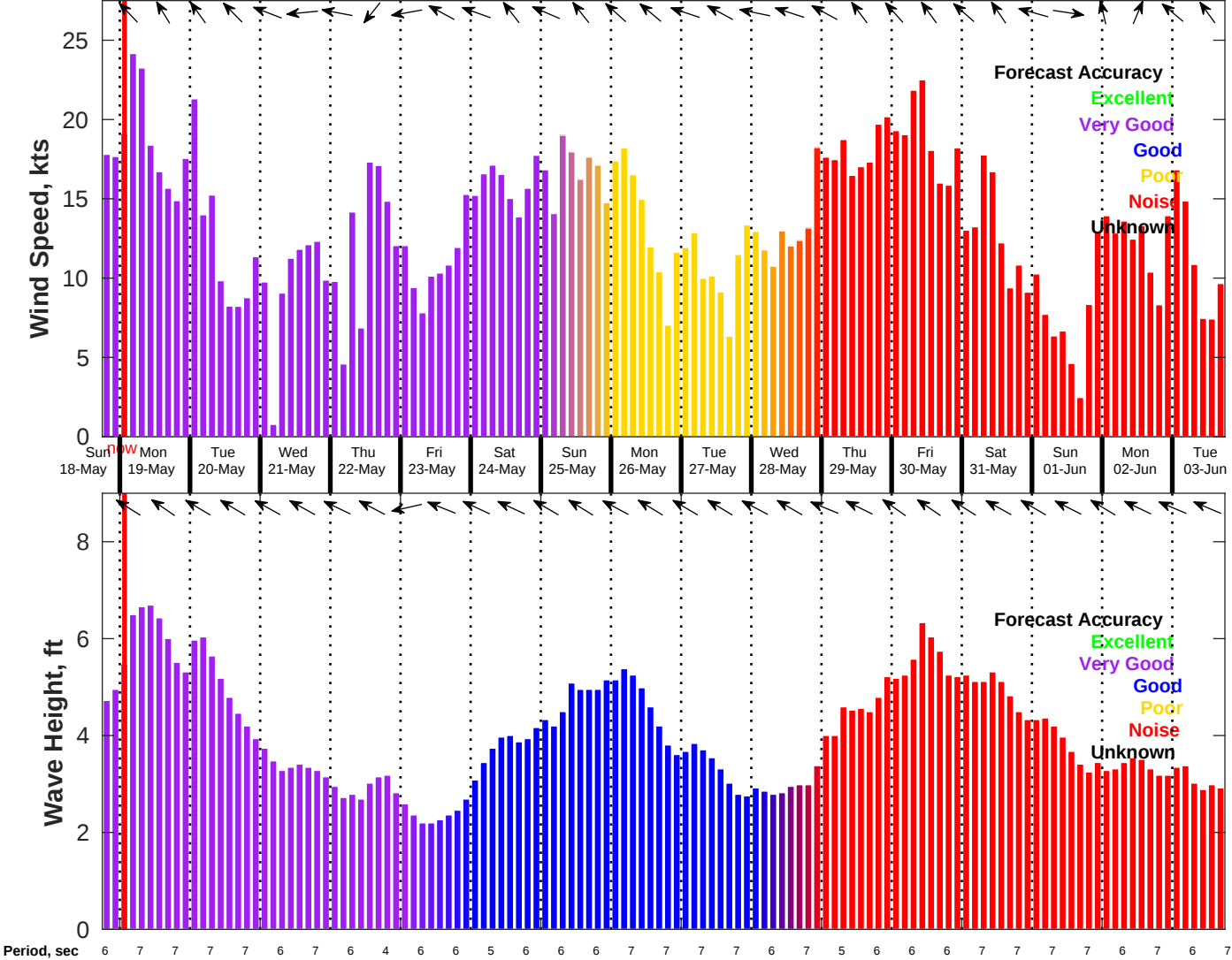
Wind & Wave Forecast for NDBC 42020 from 18-May-2025 18:00:00 to 03-Jun-2025 18:00:00
