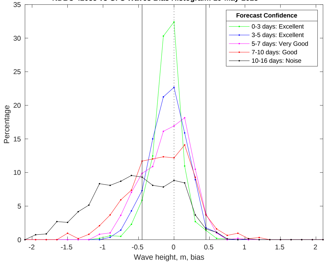
NDBC 42035 vs GFS Waves Bias Histogram: 19-May-2025
