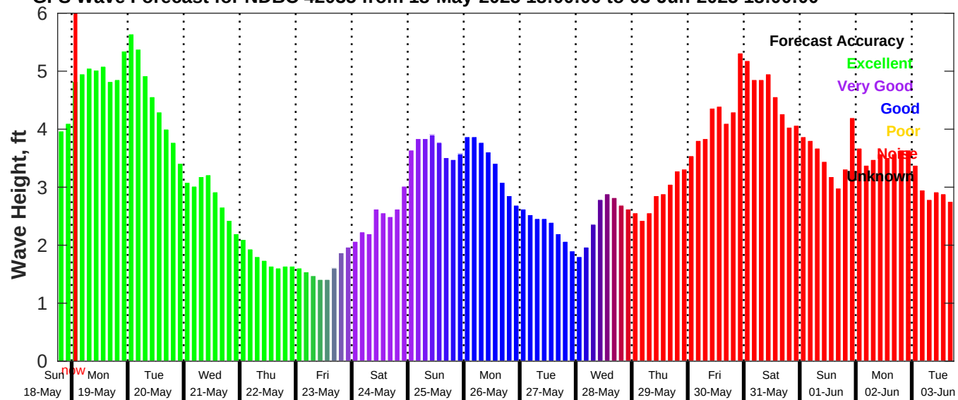
GFS Wave Forecast for NDBC 42035 from 18-May-2025 18:00:00 to 03-Jun-2025 18:00:00
