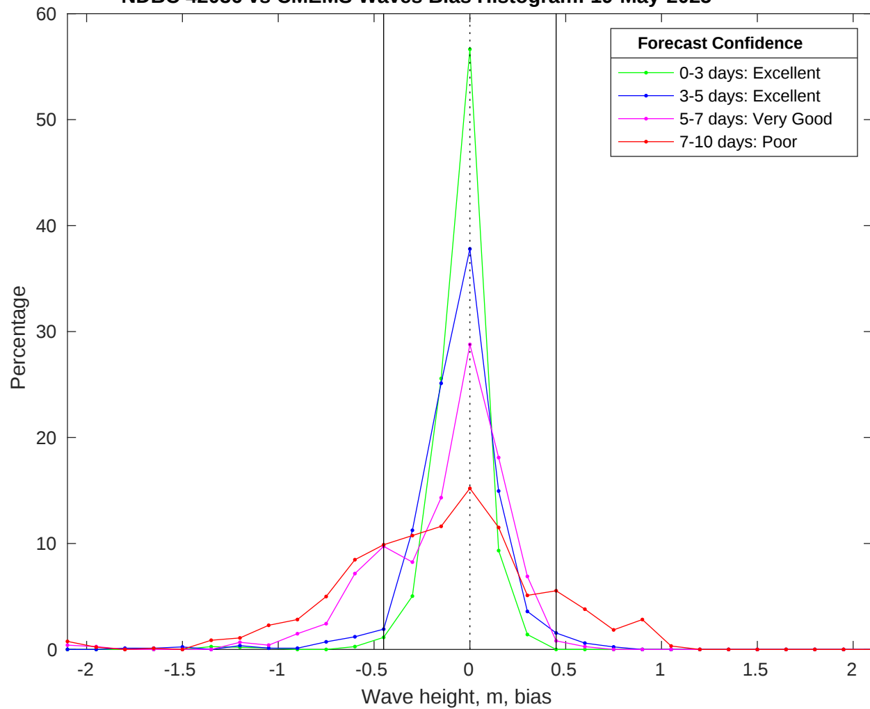
NDBC 42036 vs CMEMS Waves Bias Histogram: 19-May-2025
