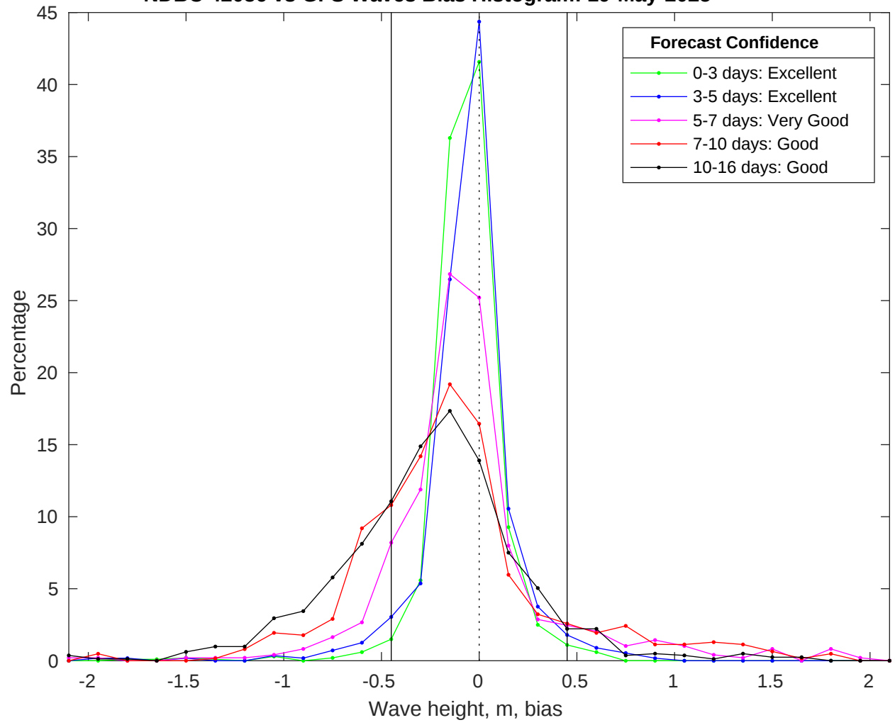
NDBC 42036 vs GFS Waves Bias Histogram: 19-May-2025
