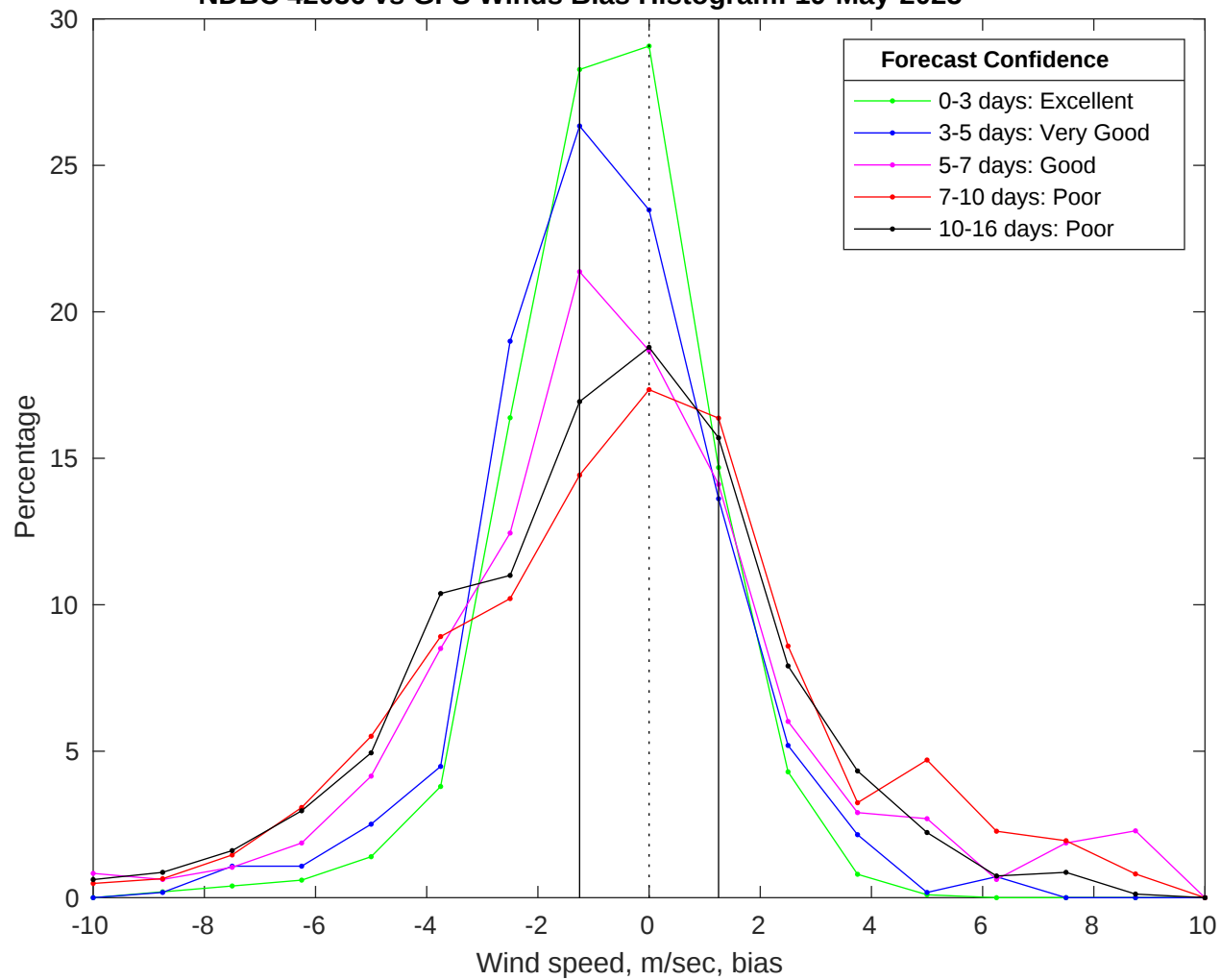
NDBC 42036 vs GFS Winds Bias Histogram: 19-May-2025
