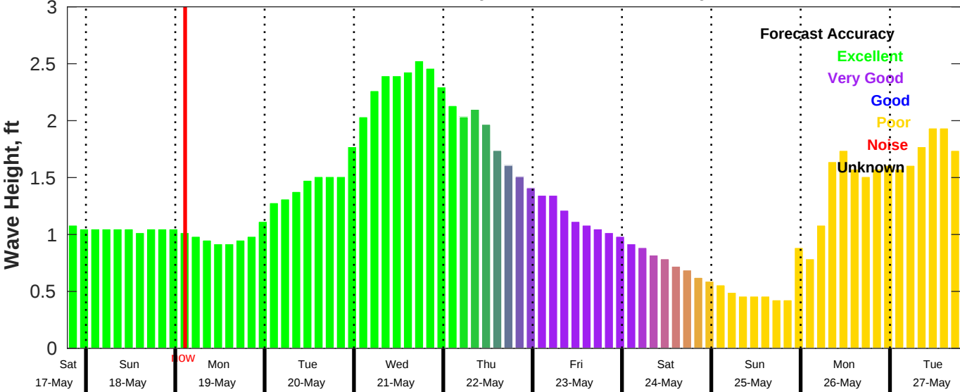
CMEMS Wave Forecast for NDBC 42036 from 17-May-2025 19:00:00 to 27-May-2025 19:00:00
