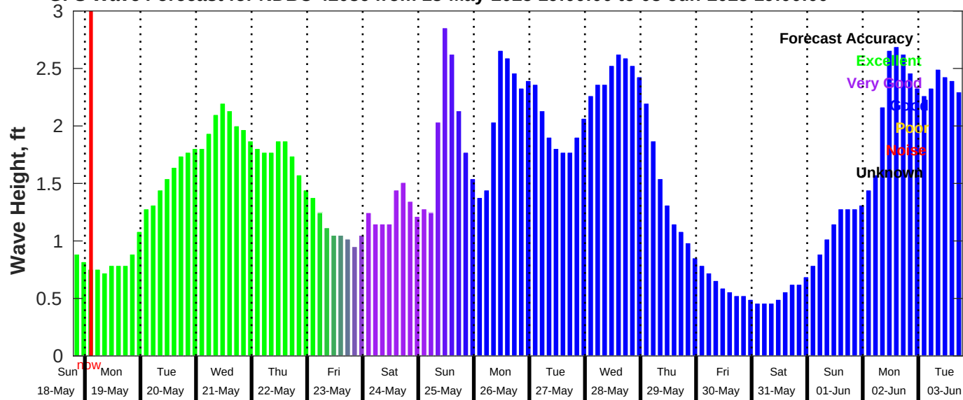
GFS Wave Forecast for NDBC 42036 from 18-May-2025 19:00:00 to 03-Jun-2025 19:00:00
