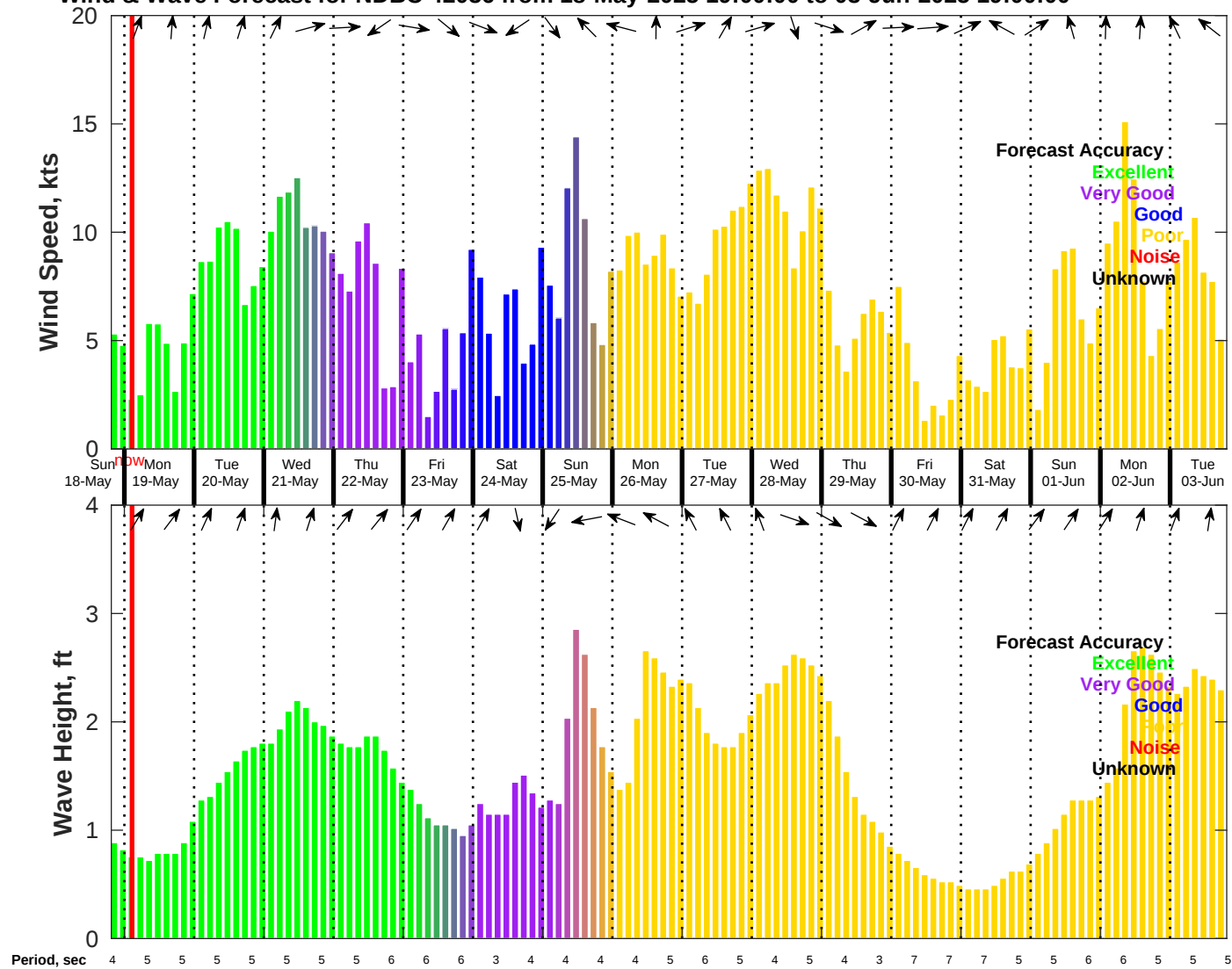
Wind & Wave Forecast for NDBC 42036 from 18-May-2025 19:00:00 to 03-Jun-2025 19:00:00
