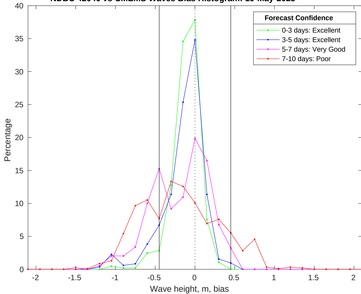
NDBC 42040 vs CMEMS Waves Bias Histogram: 19-May-2025
