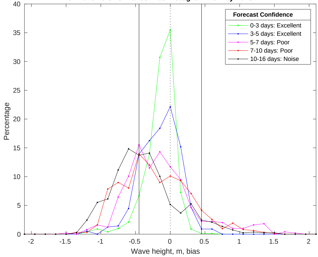
NDBC 42040 vs GFS Waves Bias Histogram: 19-May-2025
