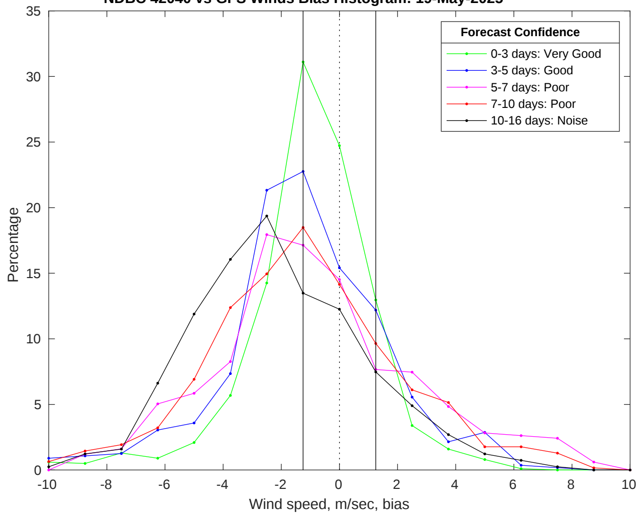
NDBC 42040 vs GFS Winds Bias Histogram: 19-May-2025
