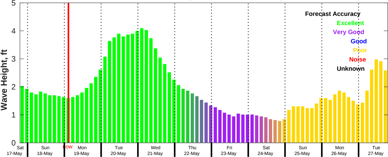
CMEMS Wave Forecast for NDBC 42040 from 17-May-2025 19:00:00 to 27-May-2025 19:00:00
