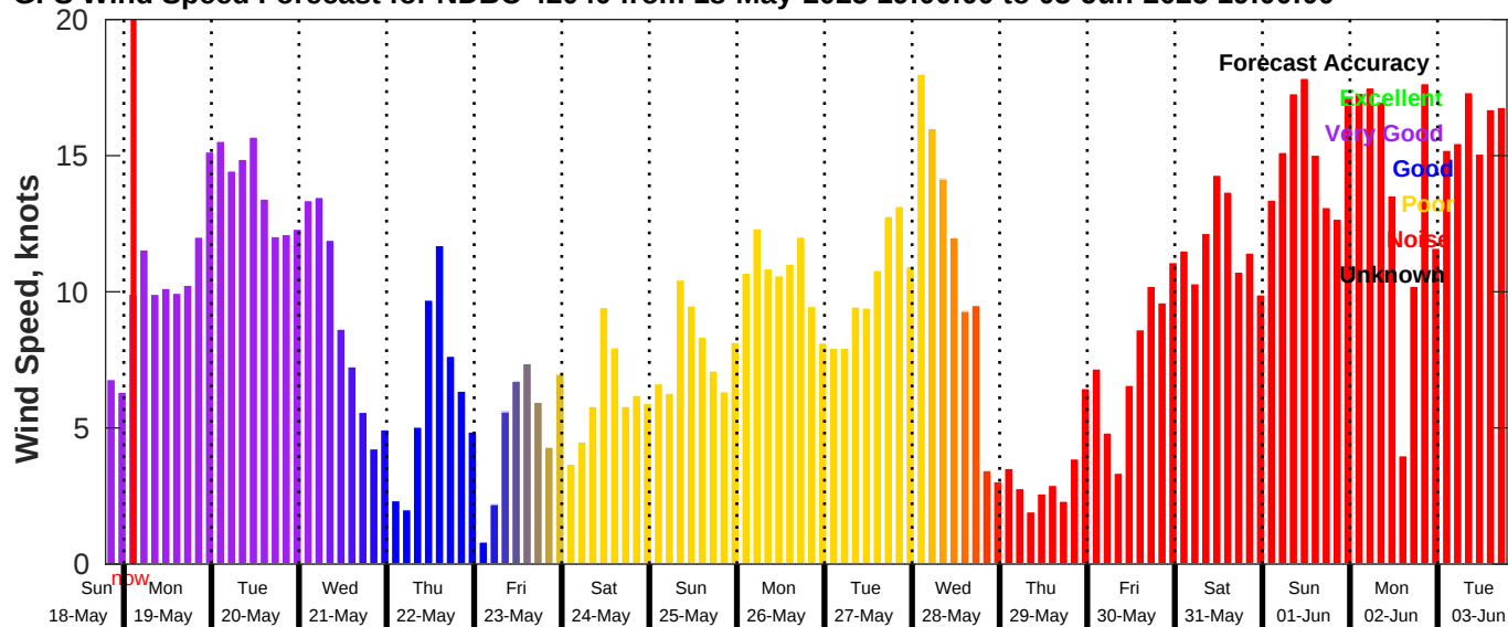
GFS Wind Speed Forecast for NDBC 42040 from 18-May-2025 19:00:00 to 03-Jun-2025 19:00:00
