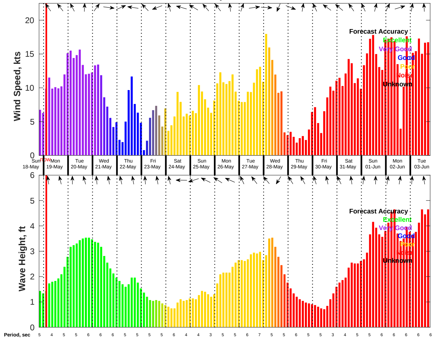
Wind & Wave Forecast for NDBC 42040 from 18-May-2025 19:00:00 to 03-Jun-2025 19:00:00
