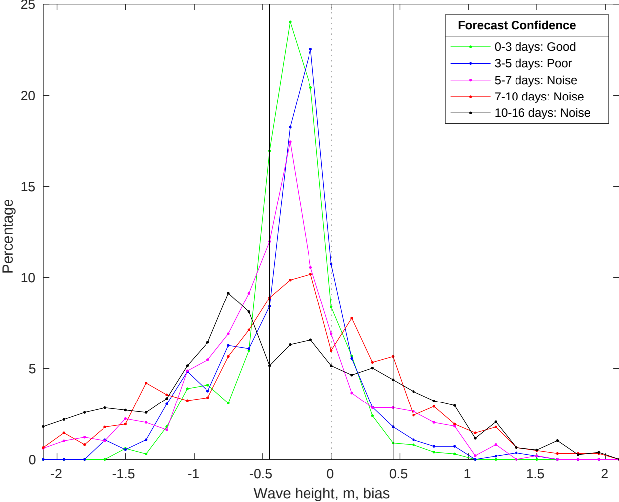
NDBC 46011 vs GFS Waves Bias Histogram: 19-May-2025
