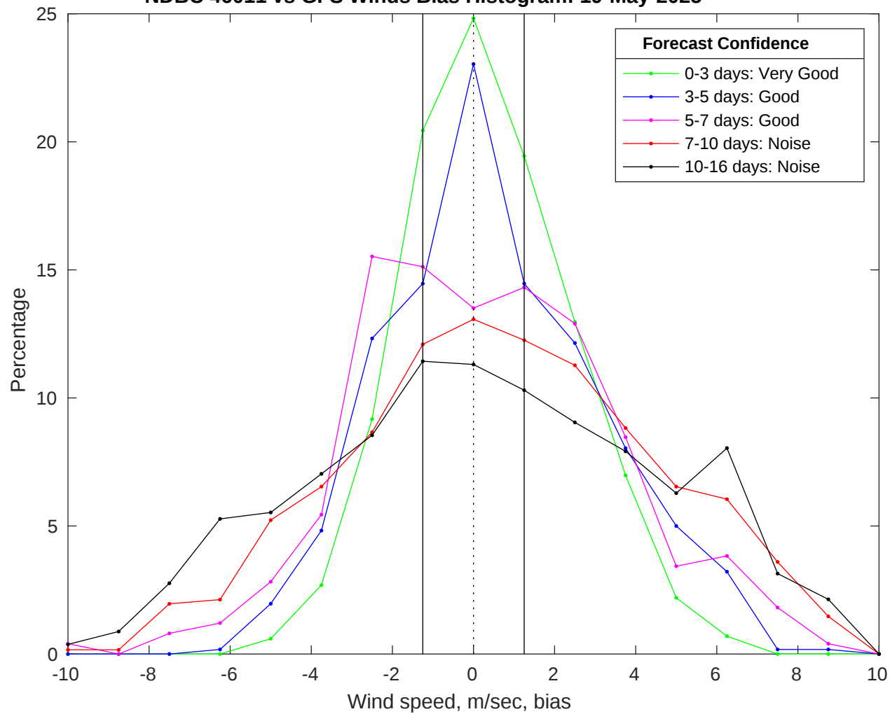
NDBC 46011 vs GFS Winds Bias Histogram: 19-May-2025
