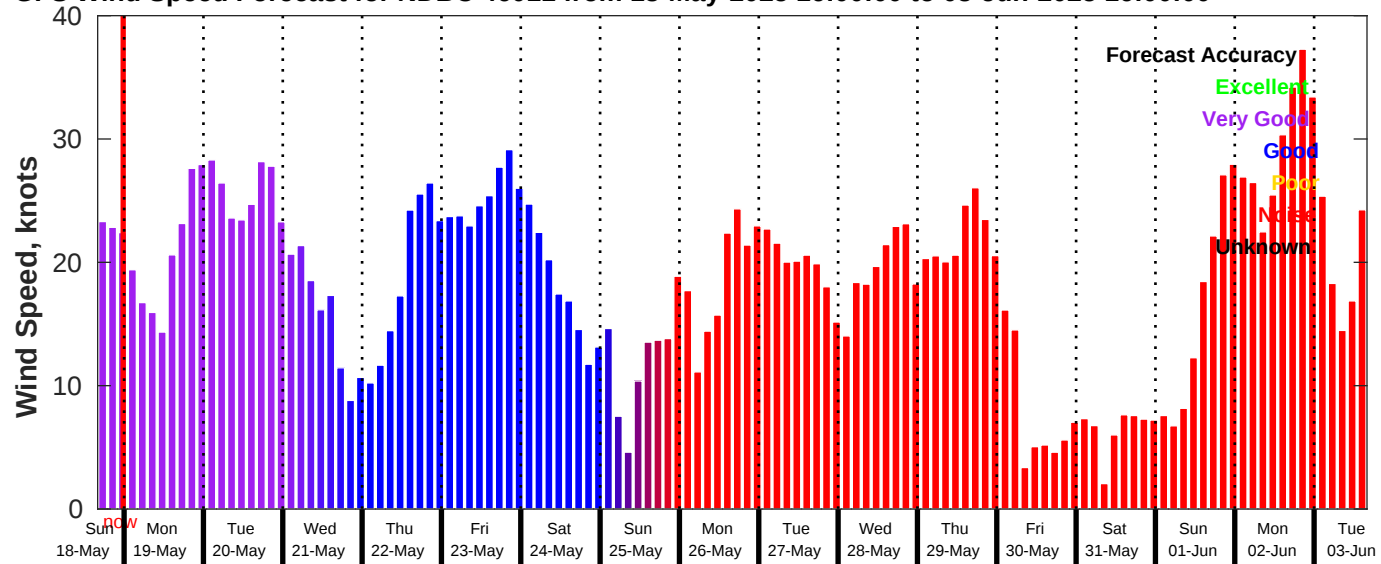
GFS Wind Speed Forecast for NDBC 46011 from 18-May-2025 16:00:00 to 03-Jun-2025 16:00:00
