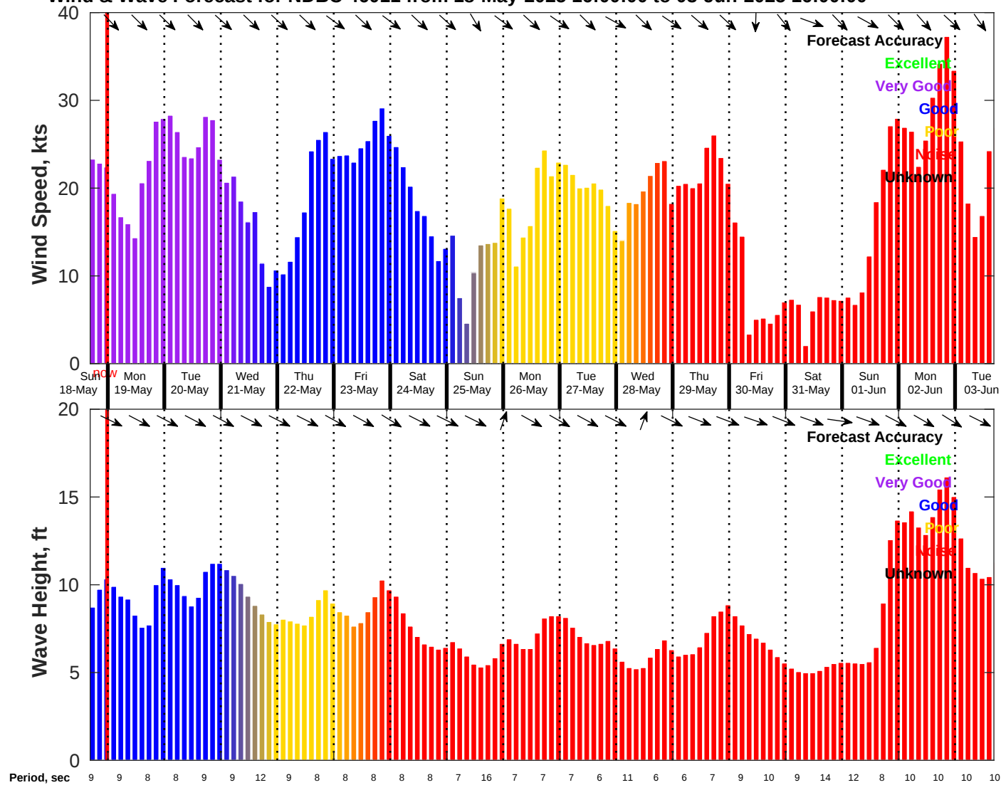
Wind & Wave Forecast for NDBC 46011 from 18-May-2025 16:00:00 to 03-Jun-2025 16:00:00
