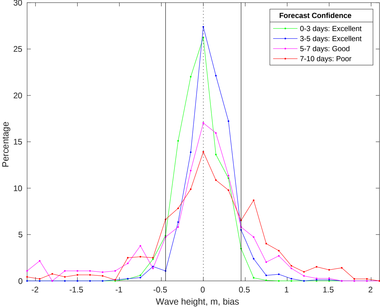
NDBC 46028 vs CMEMS Waves Bias Histogram: 19-May-2025
