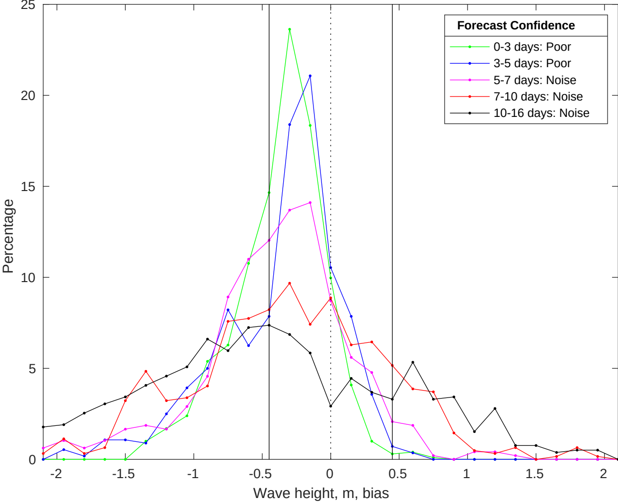
NDBC 46028 vs GFS Waves Bias Histogram: 19-May-2025
