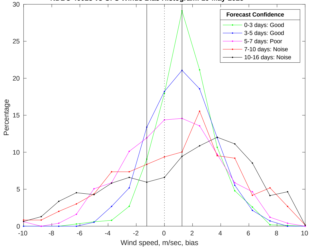
NDBC 46028 vs GFS Winds Bias Histogram: 19-May-2025
