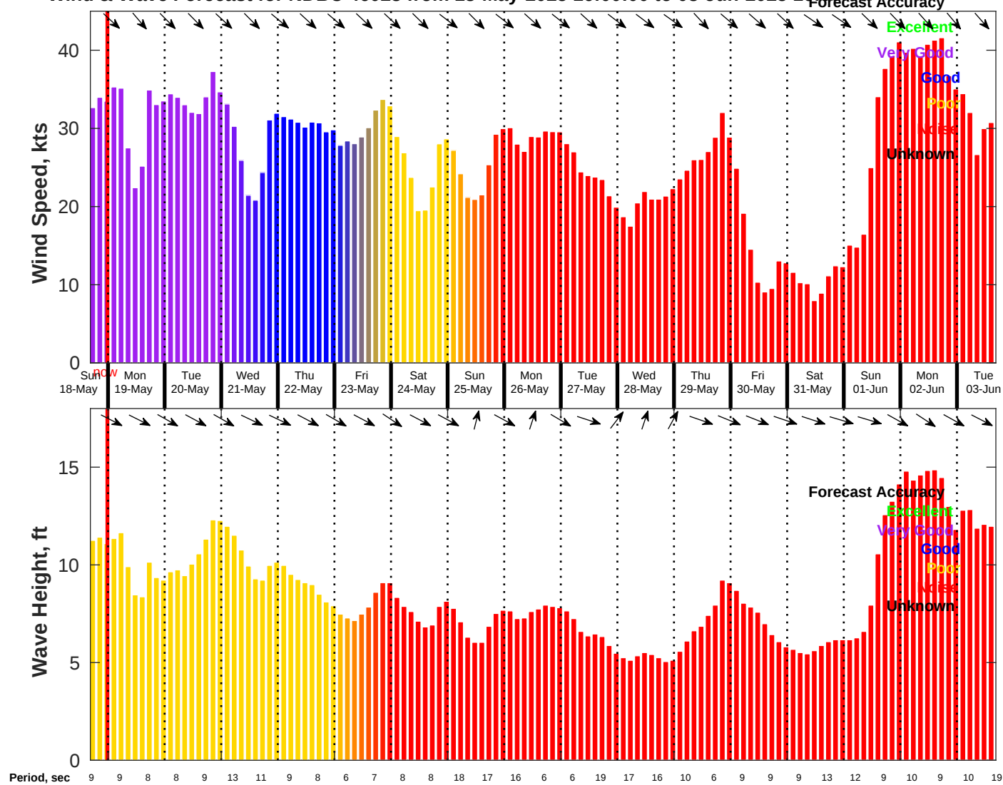
Wind & Wave Forecast for NDBC 46028 from 18-May-2025 16:00:00 to 03-Jun-2025 16:00:00
