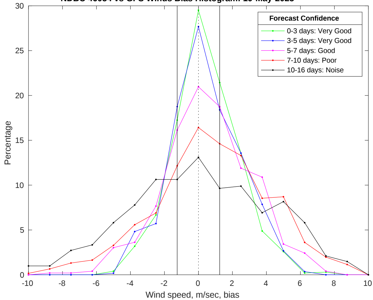
NDBC 46054 vs GFS Winds Bias Histogram: 19-May-2025
