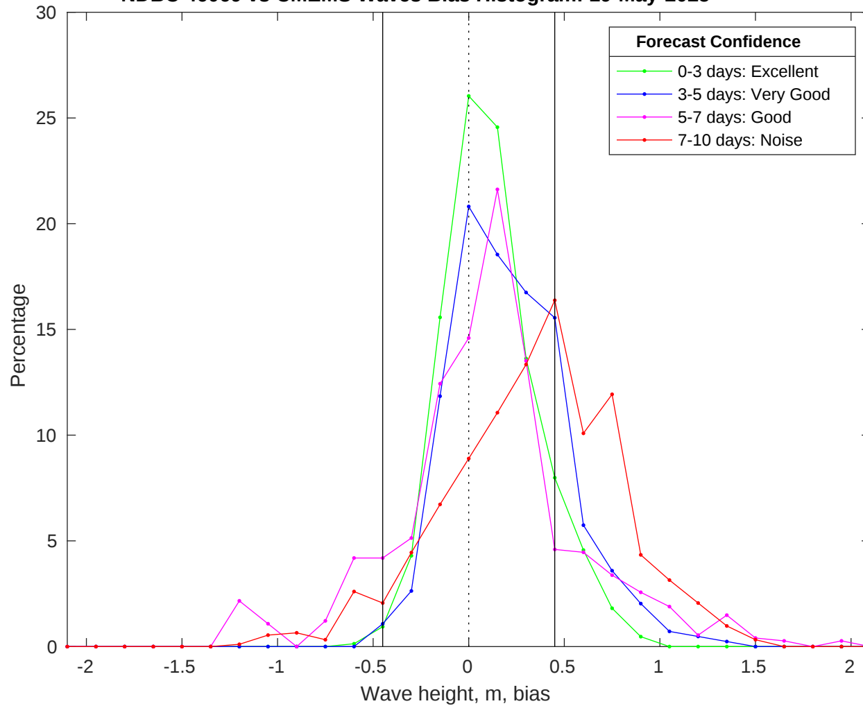
NDBC 46069 vs CMEMS Waves Bias Histogram: 19-May-2025
