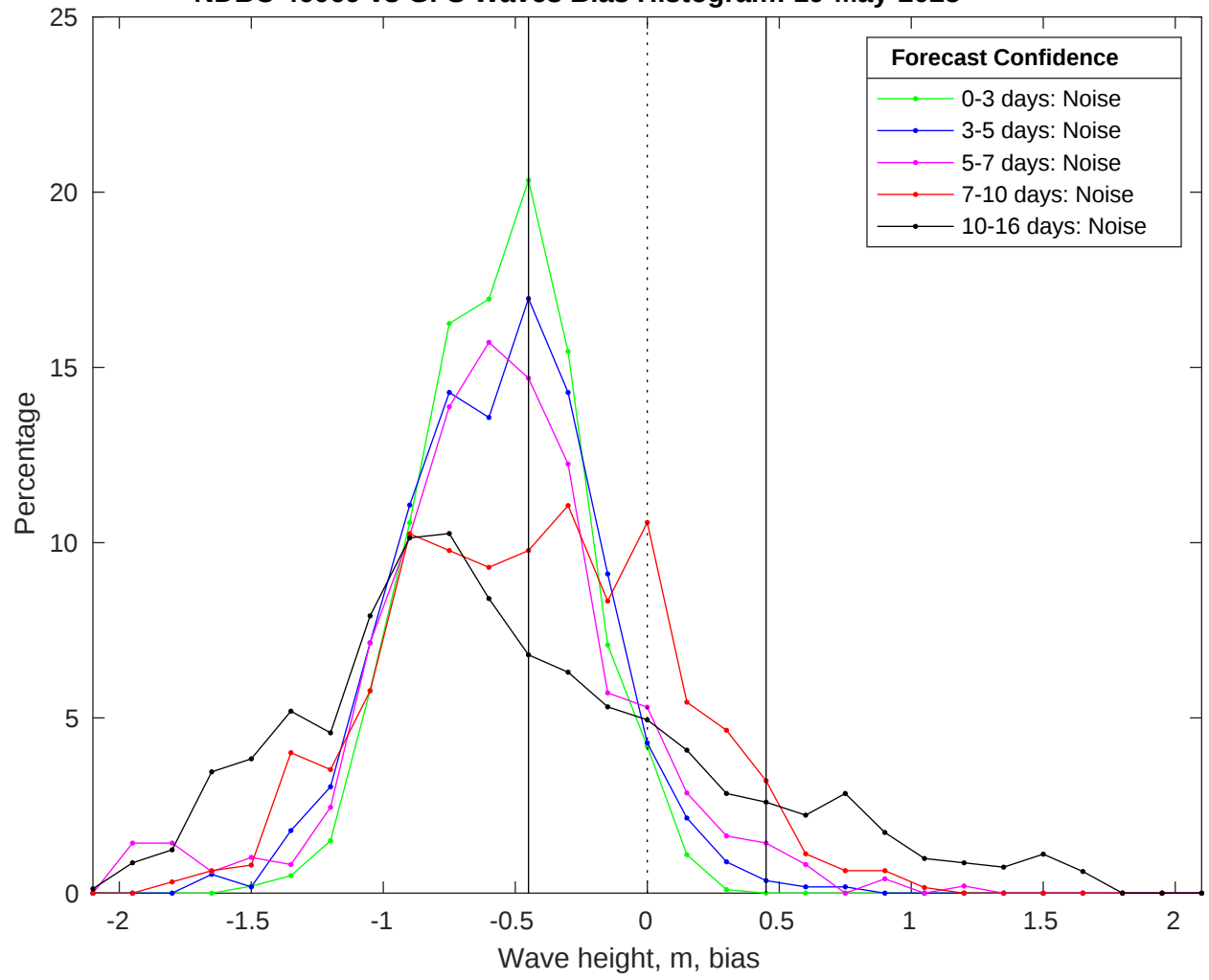
NDBC 46069 vs GFS Waves Bias Histogram: 19-May-2025
