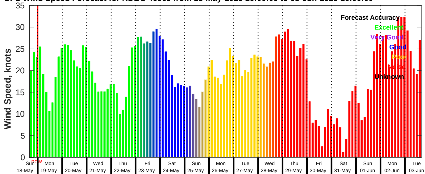
GFS Wind Speed Forecast for NDBC 46069 from 18-May-2025 16:00:00 to 03-Jun-2025 16:00:00
