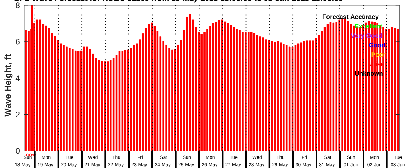
GFS Wave Forecast for NDBC 51209 from 18-May-2025 13:00:00 to 03-Jun-2025 13:00:00
