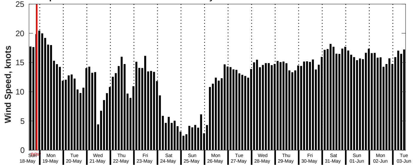
GFS Wind Speed Forecast for NDBC 51209 from 18-May-2025 13:00:00 to 03-Jun-2025 13:00:00
