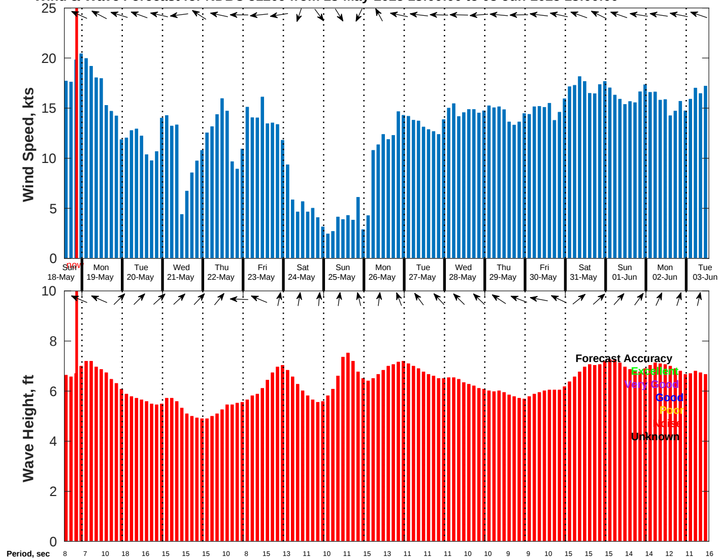
Wind & Wave Forecast for NDBC 51209 from 18-May-2025 13:00:00 to 03-Jun-2025 13:00:00
