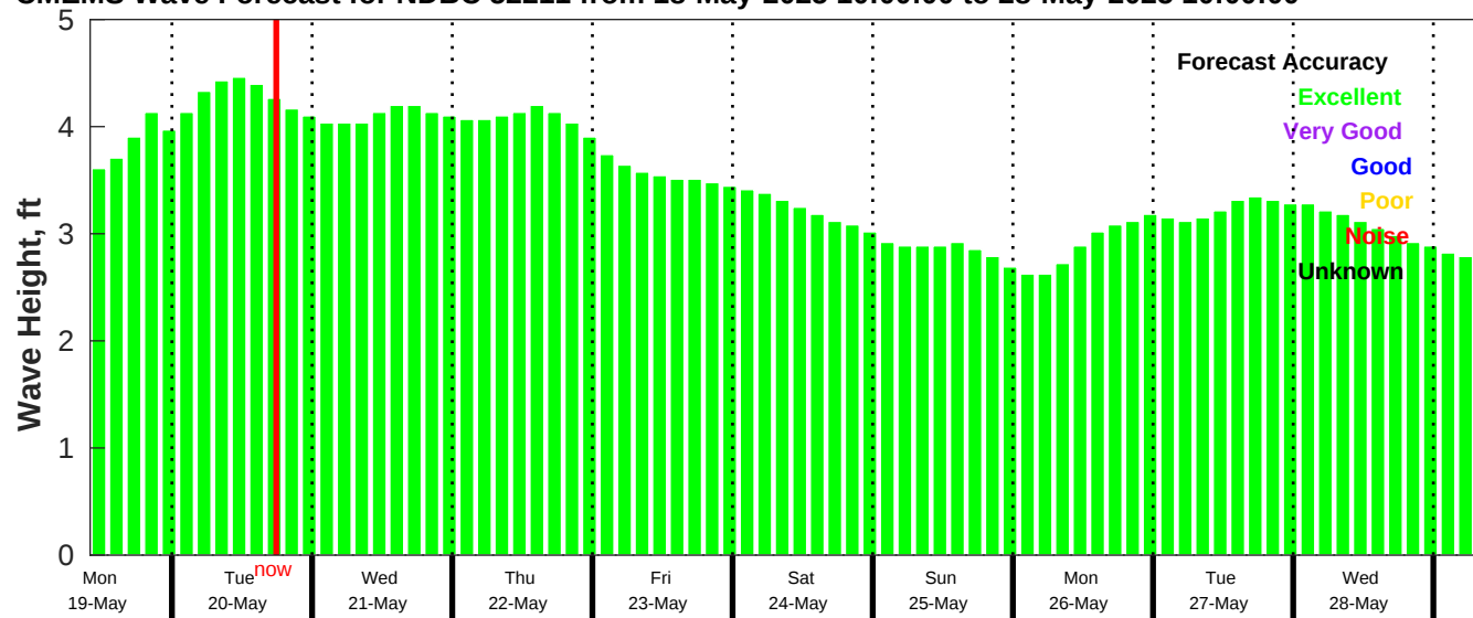
CMEMS Wave Forecast for NDBC 52211 from 18-May-2025 10:00:00 to 28-May-2025 10:00:00
