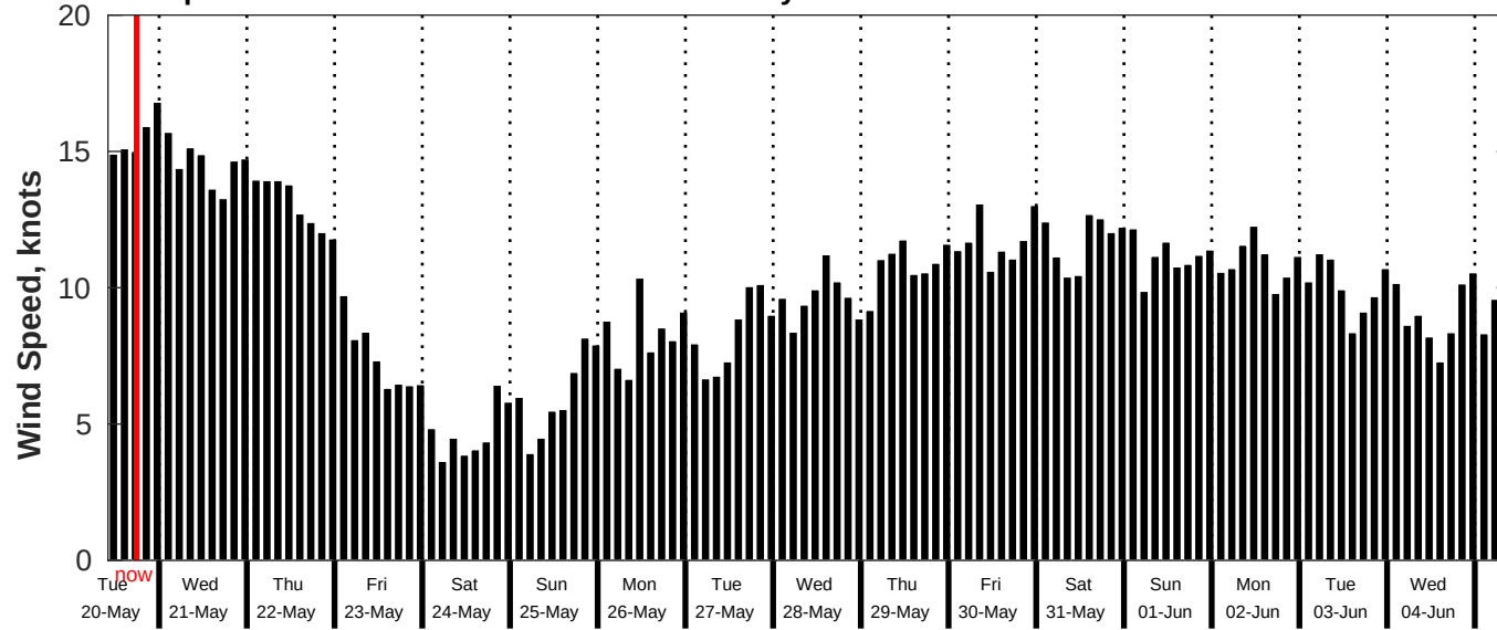
GFS Wind Speed Forecast for NDBC 52211 from 19-May-2025 10:00:00 to 04-Jun-2025 10:00:00
