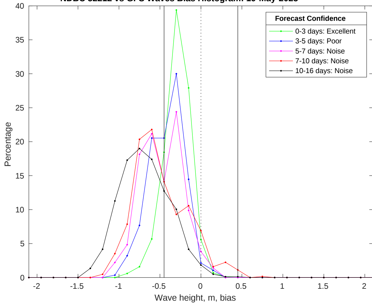
NDBC 52212 vs GFS Waves Bias Histogram: 19-May-2025
