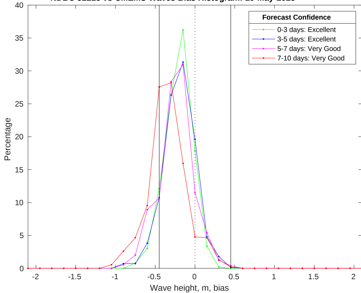
NDBC 52213 vs CMEMS Waves Bias Histogram: 19-May-2025
