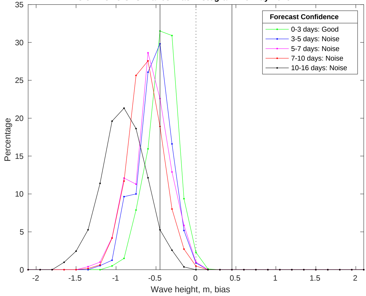
NDBC 52213 vs GFS Waves Bias Histogram: 19-May-2025
