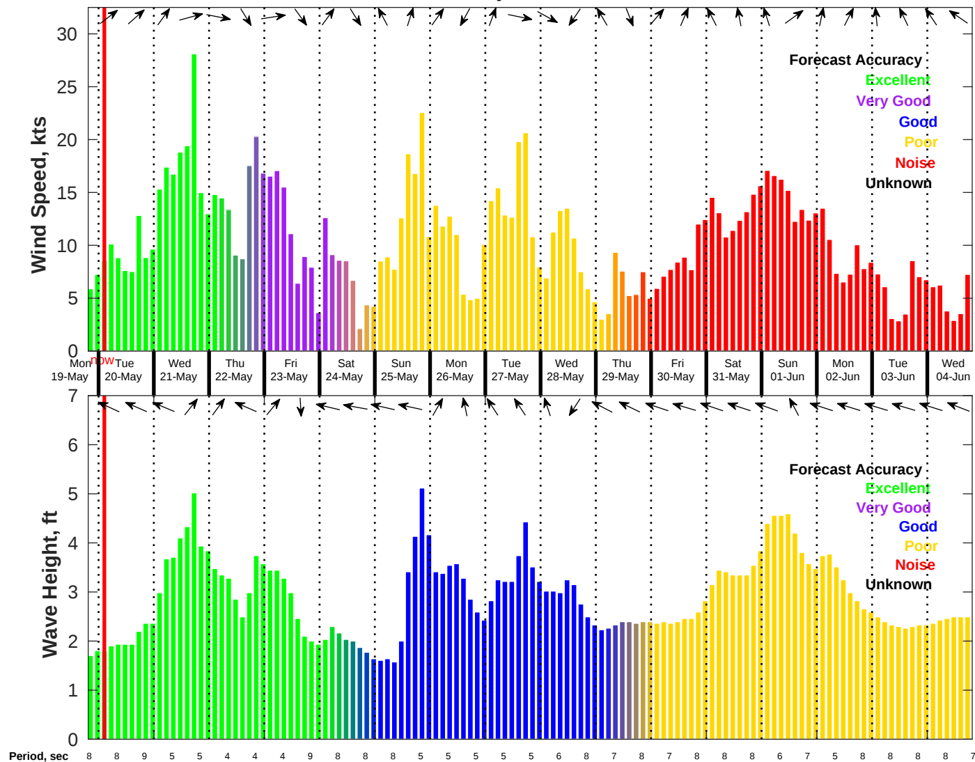
Wind & Wave Forecast for NDBC 41004 from 19-May-2025 19:00:00 to 04-Jun-2025 19:00:00
