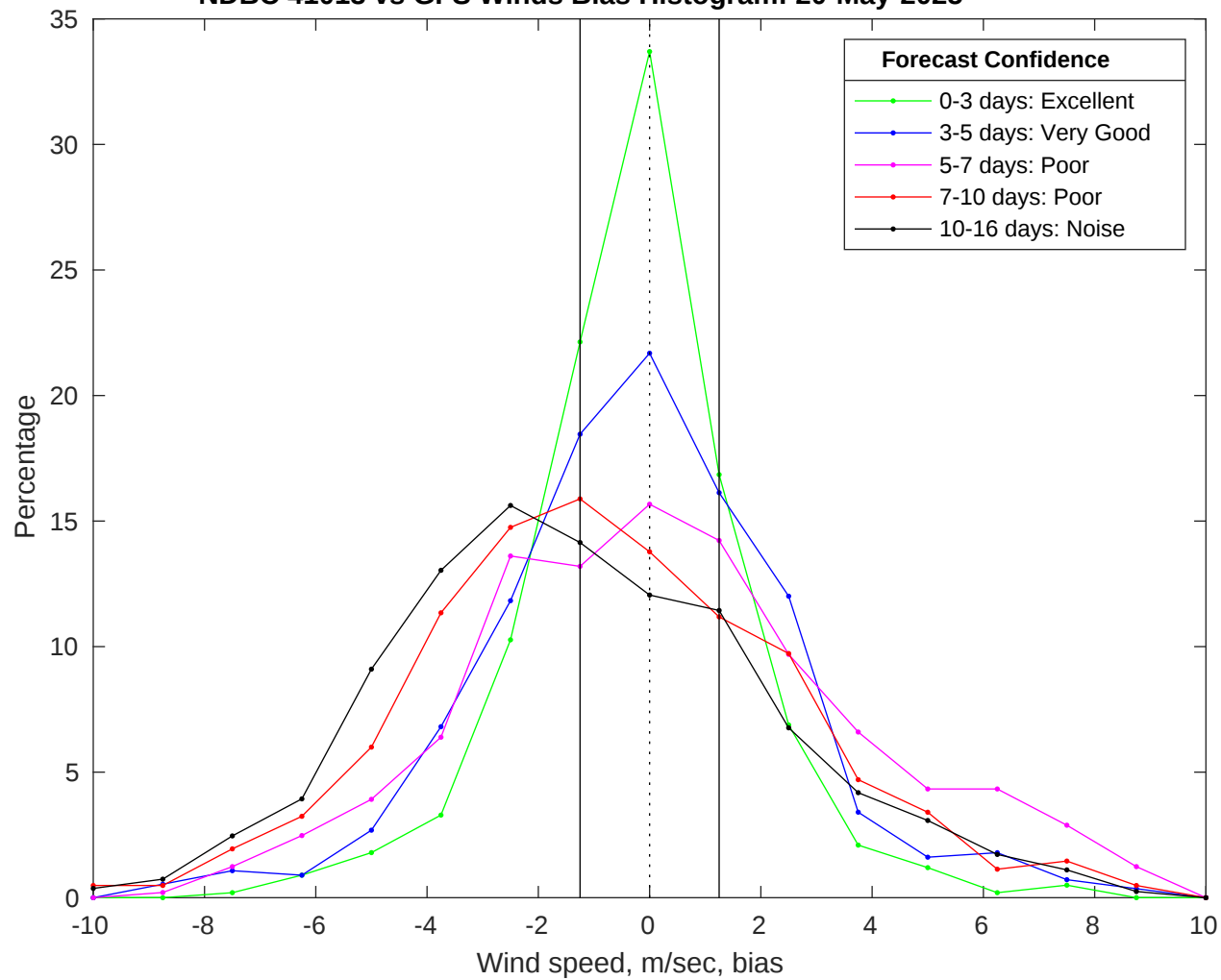
NDBC 41013 vs GFS Winds Bias Histogram: 20-May-2025
