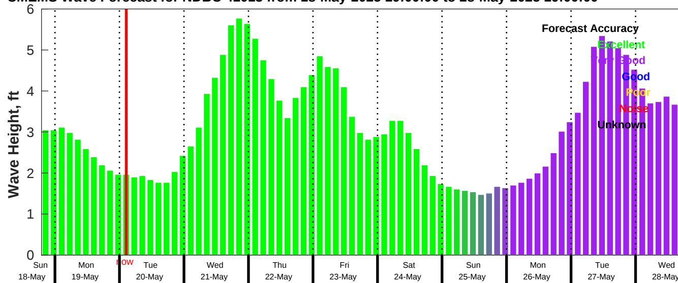
CMEMS Wave Forecast for NDBC 41013 from 18-May-2025 19:00:00 to 28-May-2025 19:00:00
