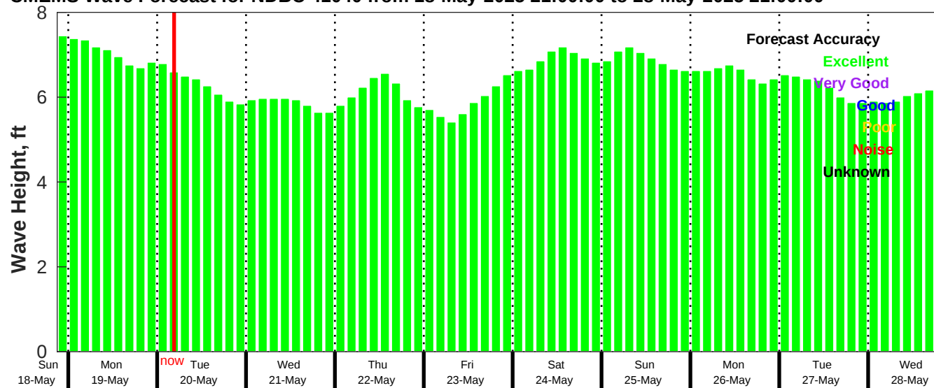
CMEMS Wave Forecast for NDBC 41040 from 18-May-2025 21:00:00 to 28-May-2025 21:00:00
