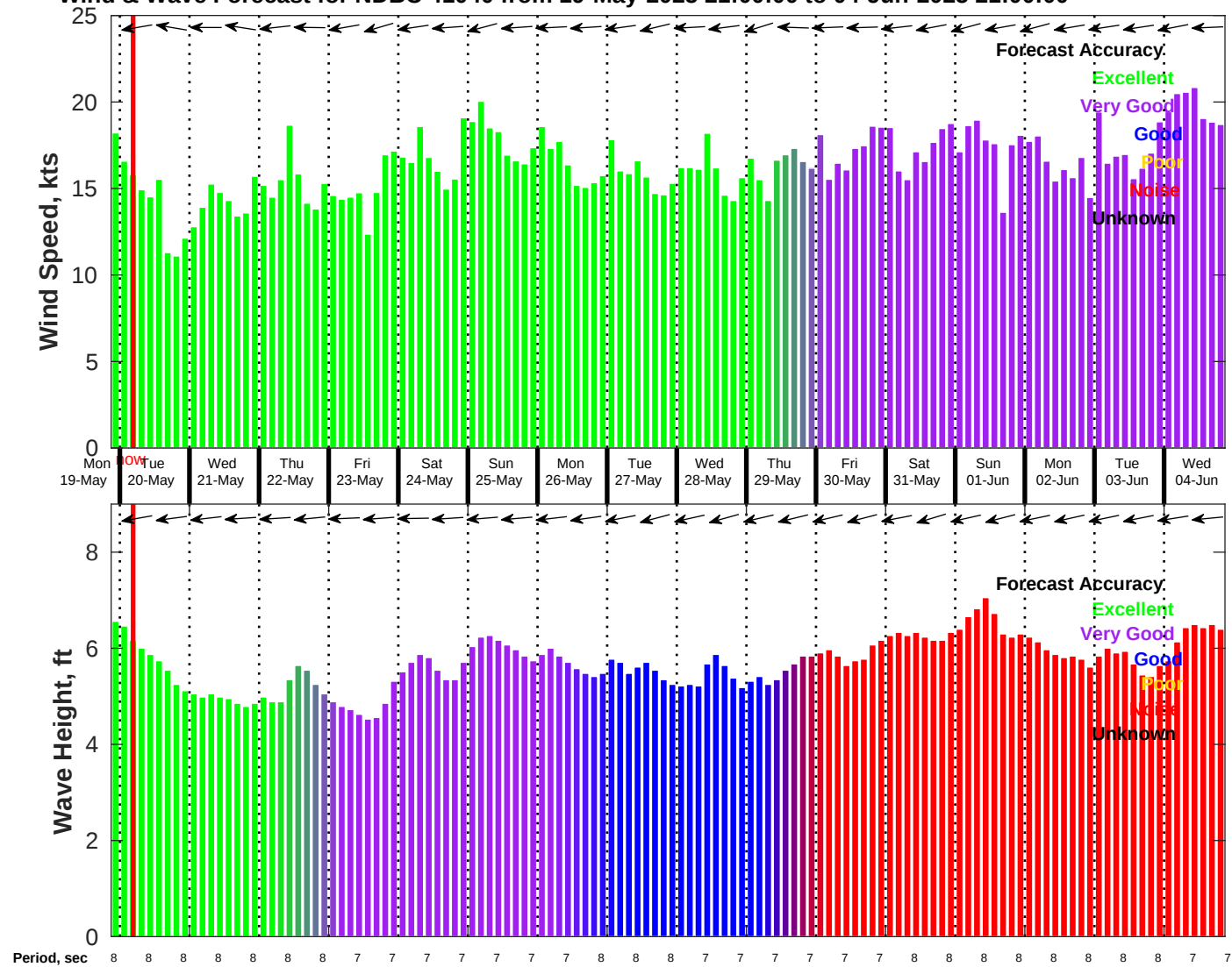
Wind & Wave Forecast for NDBC 41040 from 19-May-2025 21:00:00 to 04-Jun-2025 21:00:00
