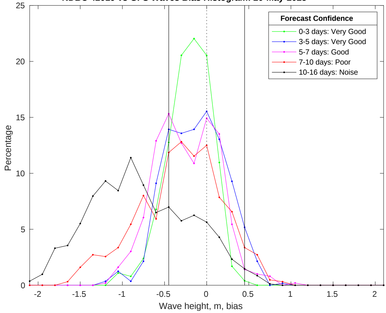
NDBC 42019 vs GFS Waves Bias Histogram: 20-May-2025
