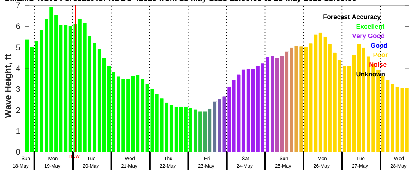
CMEMS Wave Forecast for NDBC 42019 from 18-May-2025 18:00:00 to 28-May-2025 18:00:00
