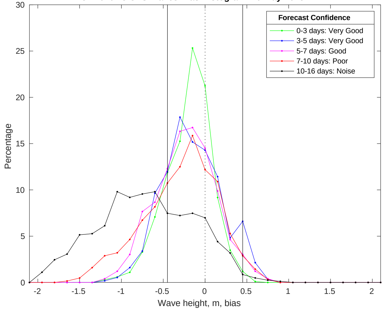
NDBC 42020 vs GFS Waves Bias Histogram: 20-May-2025
