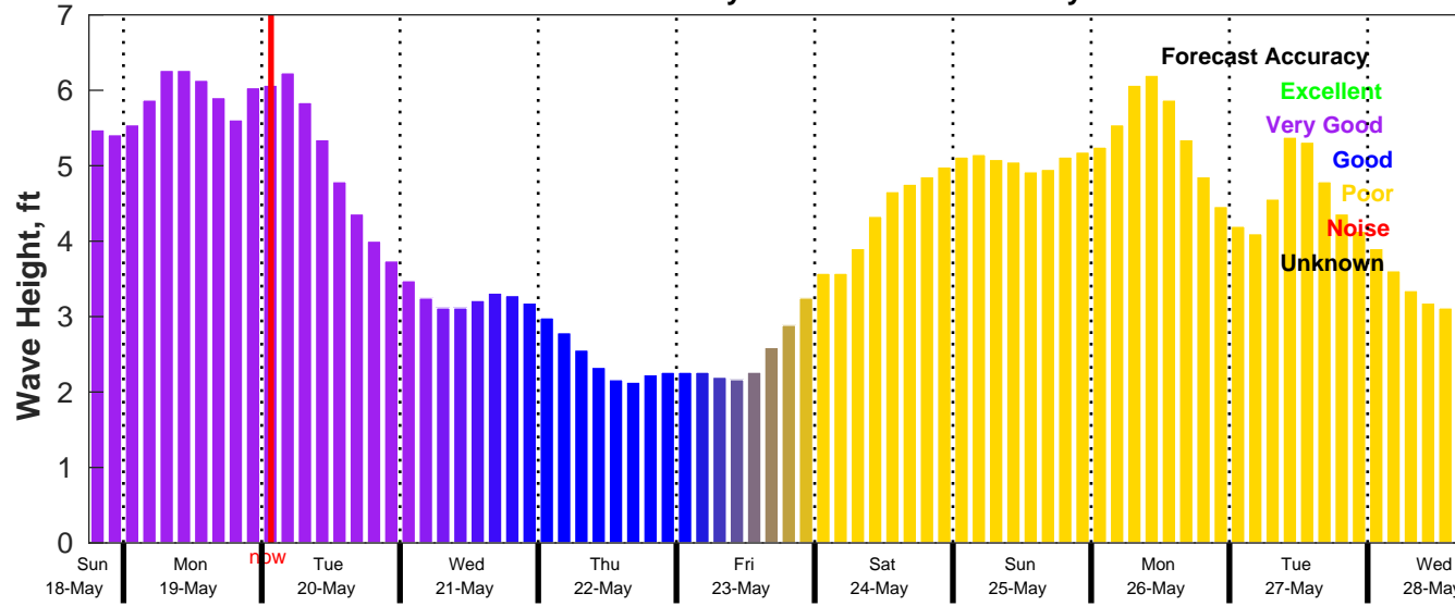
CMEMS Wave Forecast for NDBC 42020 from 18-May-2025 18:00:00 to 28-May-2025 18:00:00
