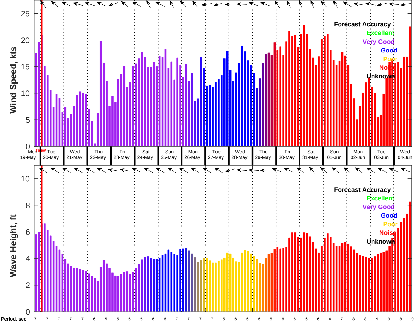
Wind & Wave Forecast for NDBC 42020 from 19-May-2025 18:00:00 to 04-Jun-2025 18:00:00
