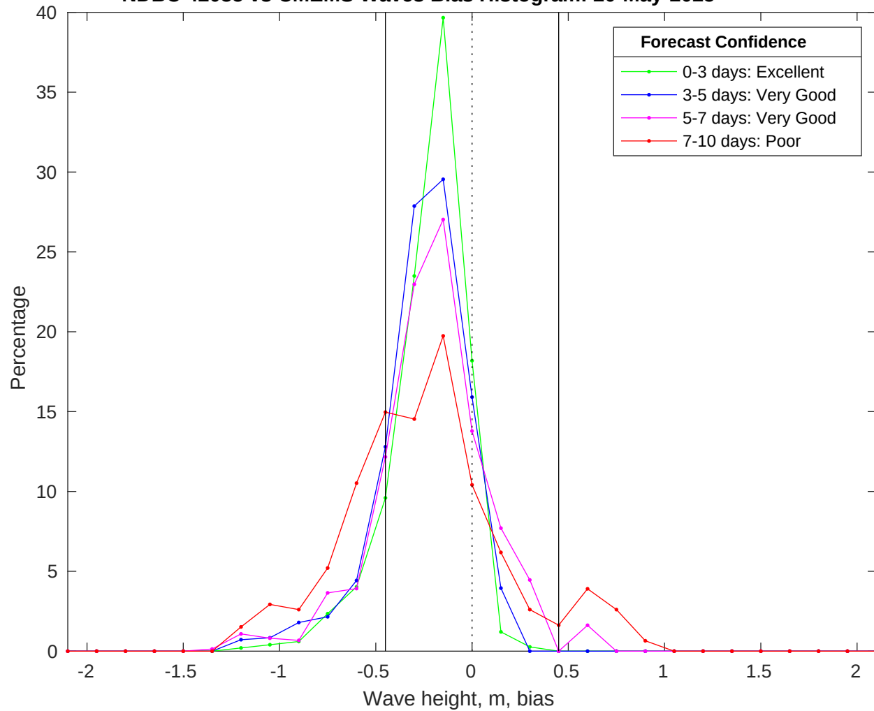
NDBC 42035 vs CMEMS Waves Bias Histogram: 20-May-2025
