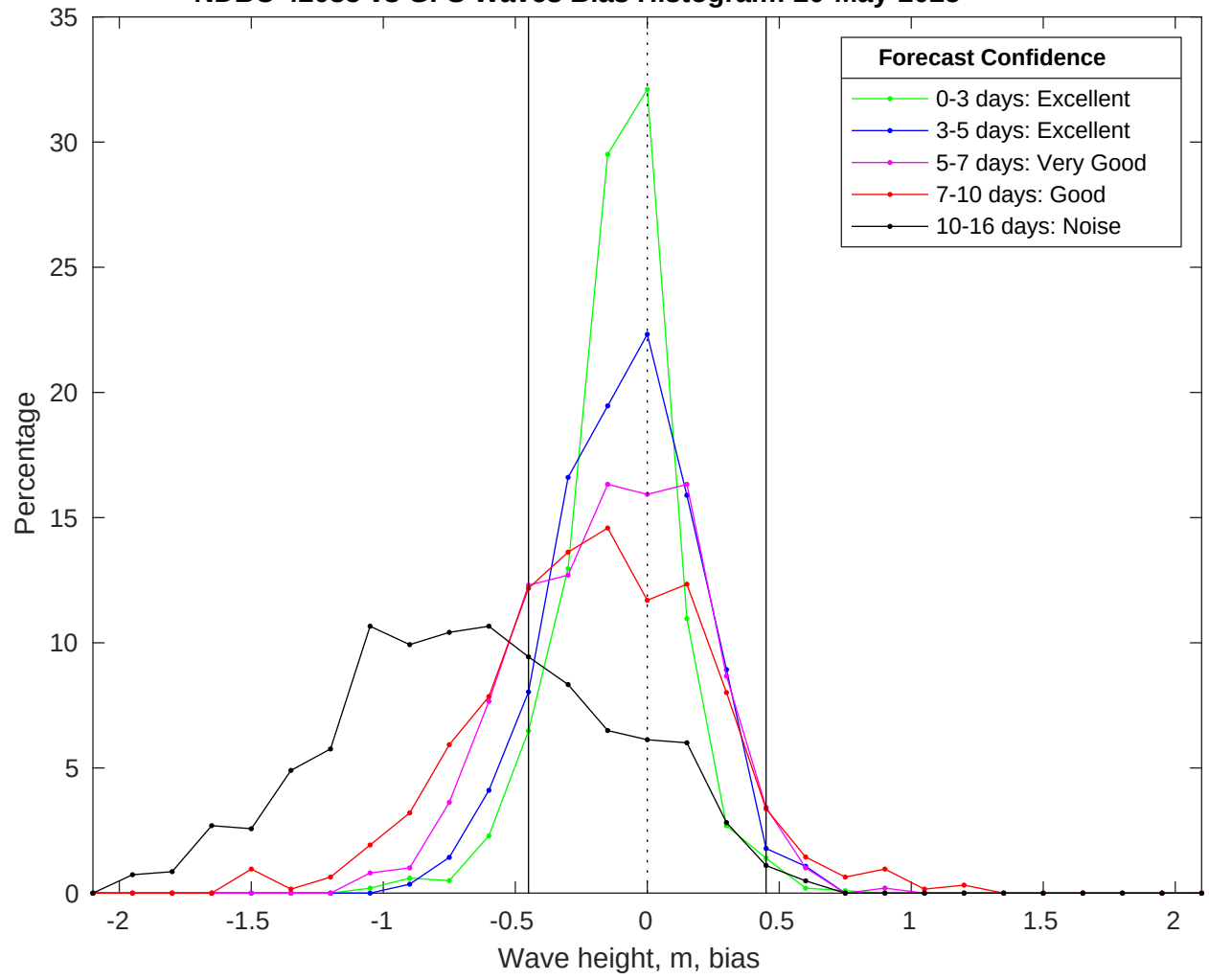
NDBC 42035 vs GFS Waves Bias Histogram: 20-May-2025
