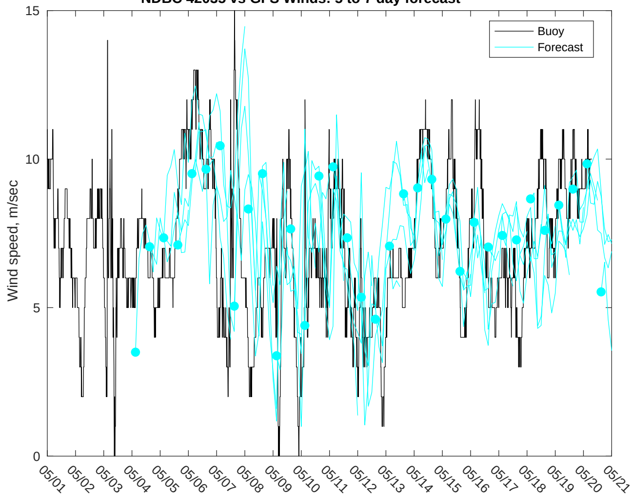
NDBC 42035 vs GFS Winds: 5 to 7 day forecast
